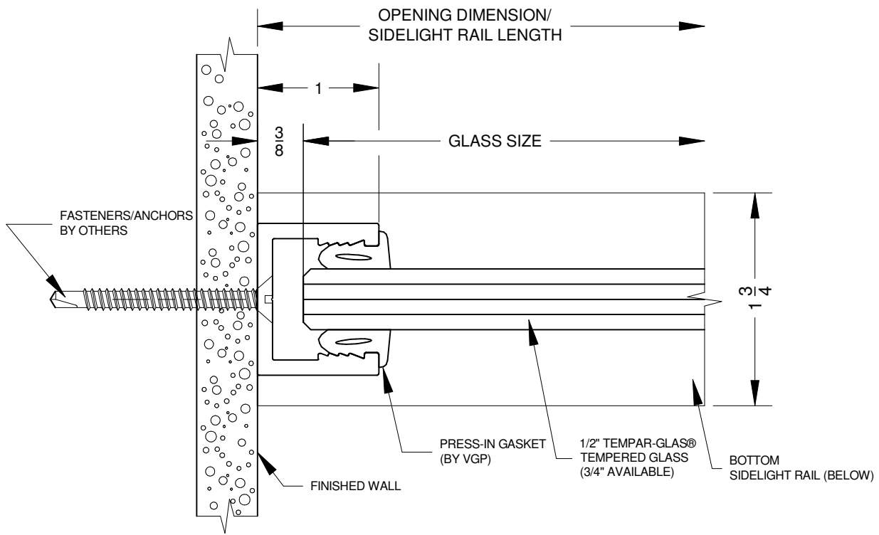
(A) - PLAN DETAIL AT SIDELIGHT JAMB w/ BOTTOM RAILS
