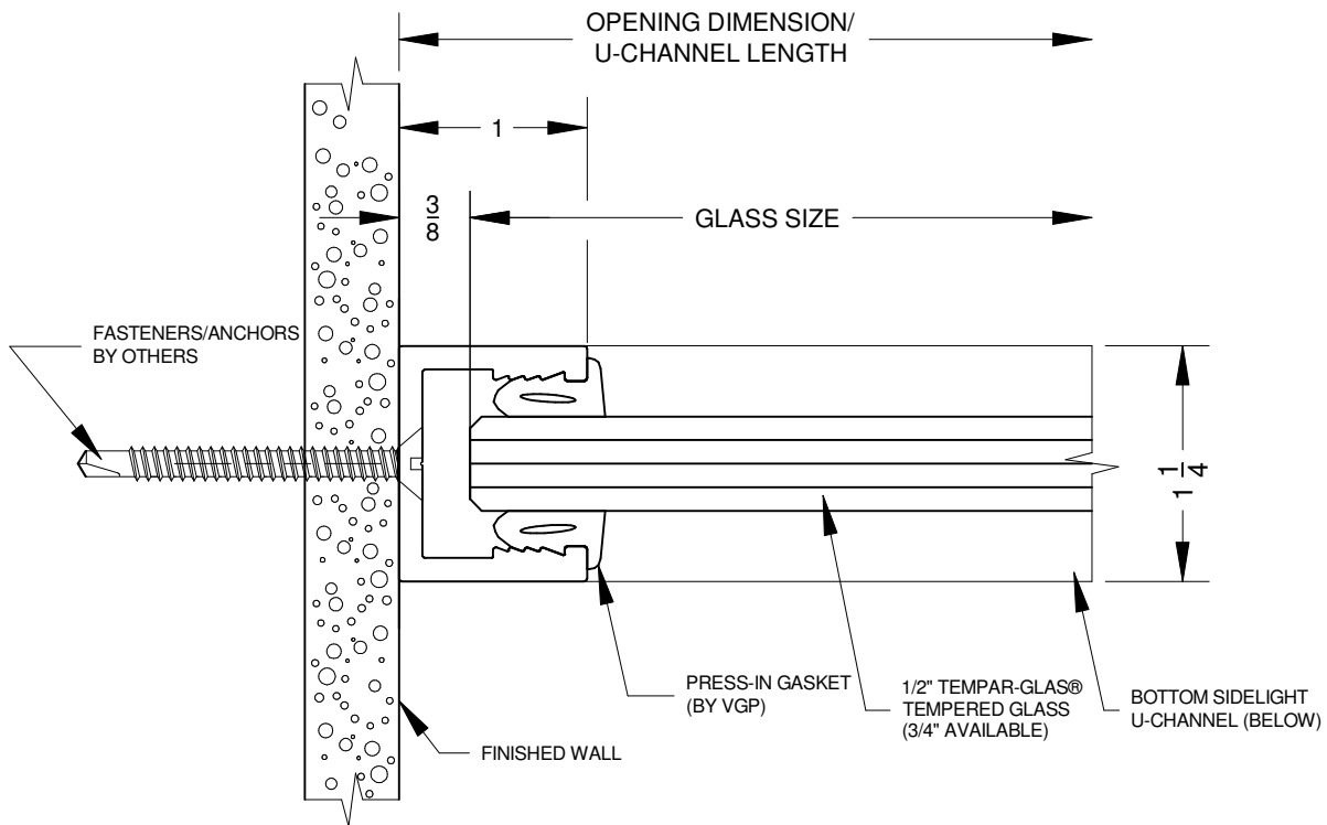
(B) - PLAN DETAIL AT SIDELIGHT JAMB w/ BOTTOM U-CHANNEL
