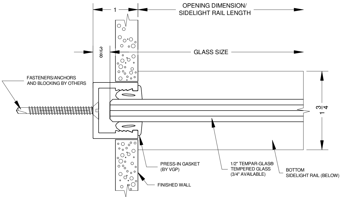
(A) - PLAN DETAIL AT SIDELIGHT JAMB w/ BOTTOM RAILS
