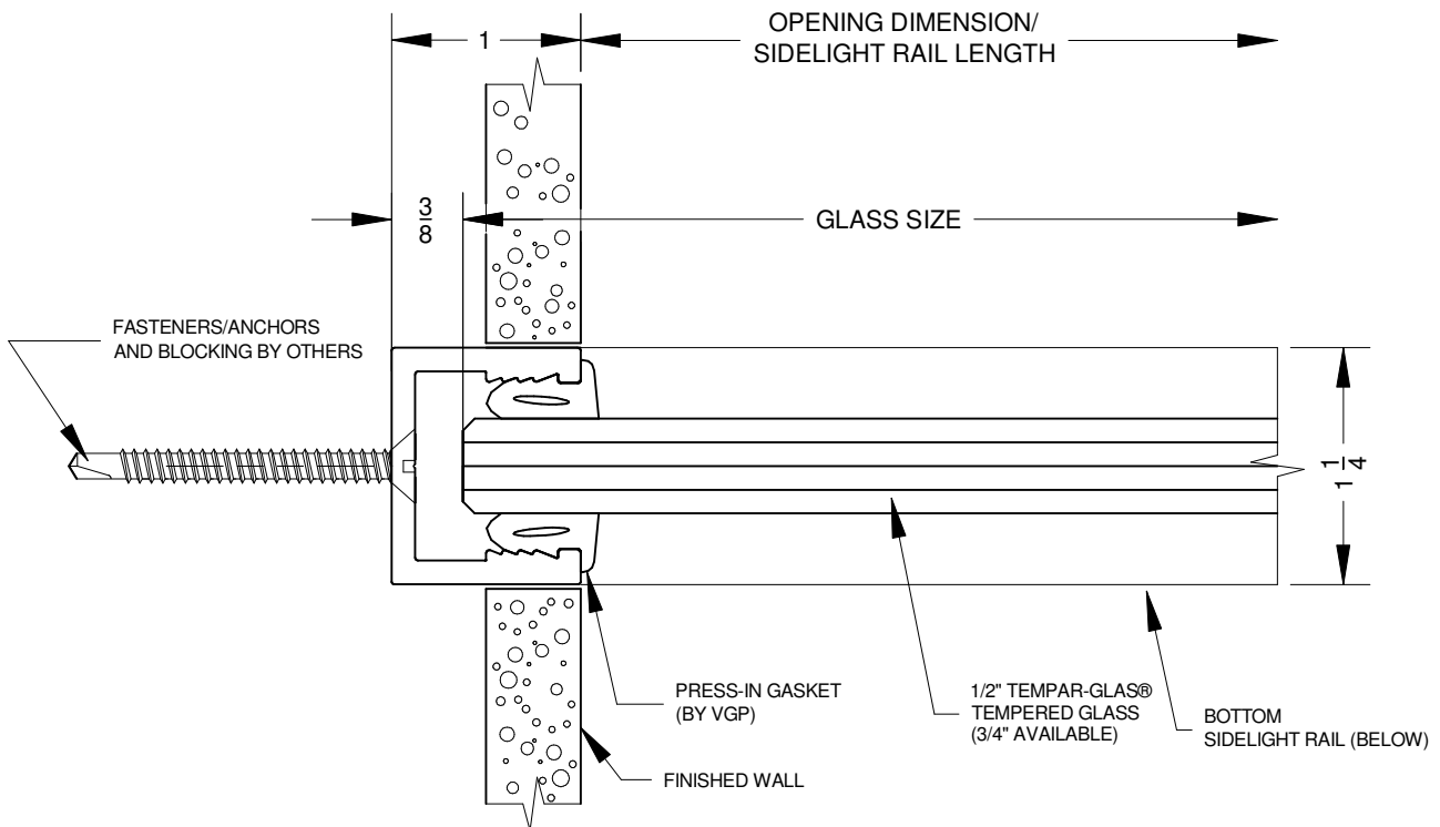
(B) - PLAN DETAIL AT SIDELIGHT JAMB w/ BOTTOM U-CHANNEL
