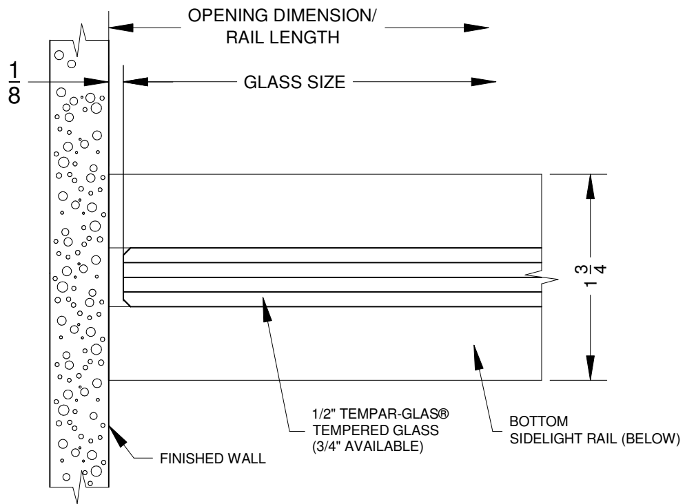
(A) - PLAN DETAIL AT SIDELIGHT JAMB w/ BOTTOM RAILS
