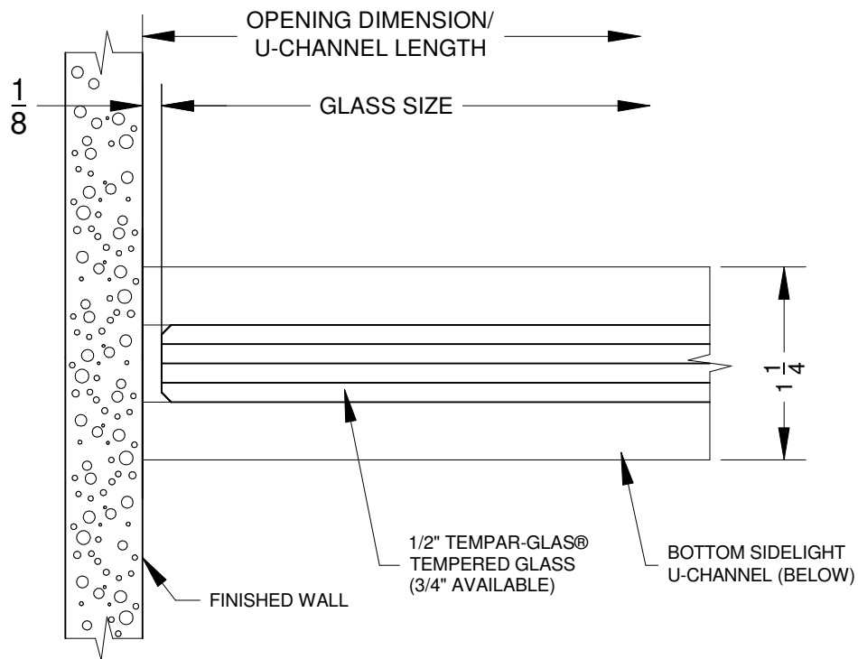
(B) - PLAN DETAIL AT SIDELIGHT JAMB w/ BOTTOM U-CHANNEL
