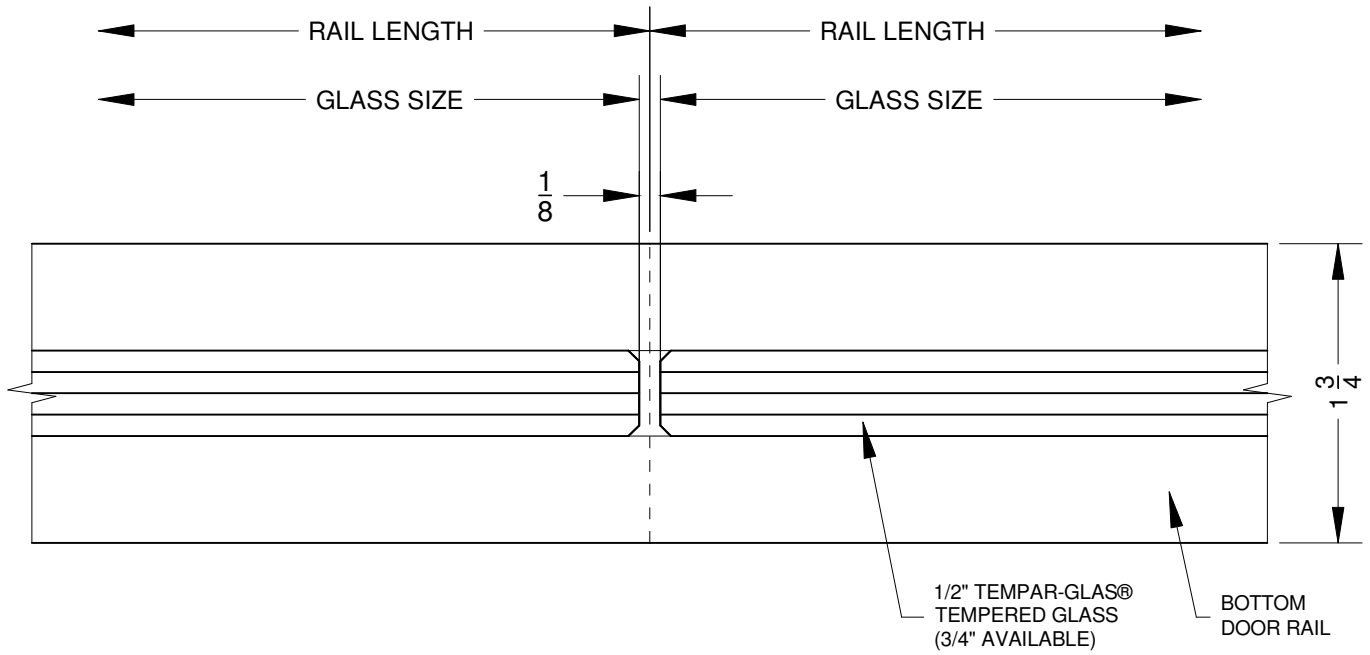
(A) - PLAN DETAIL AT MEETING SIDELIGHTS w/ RAILS
