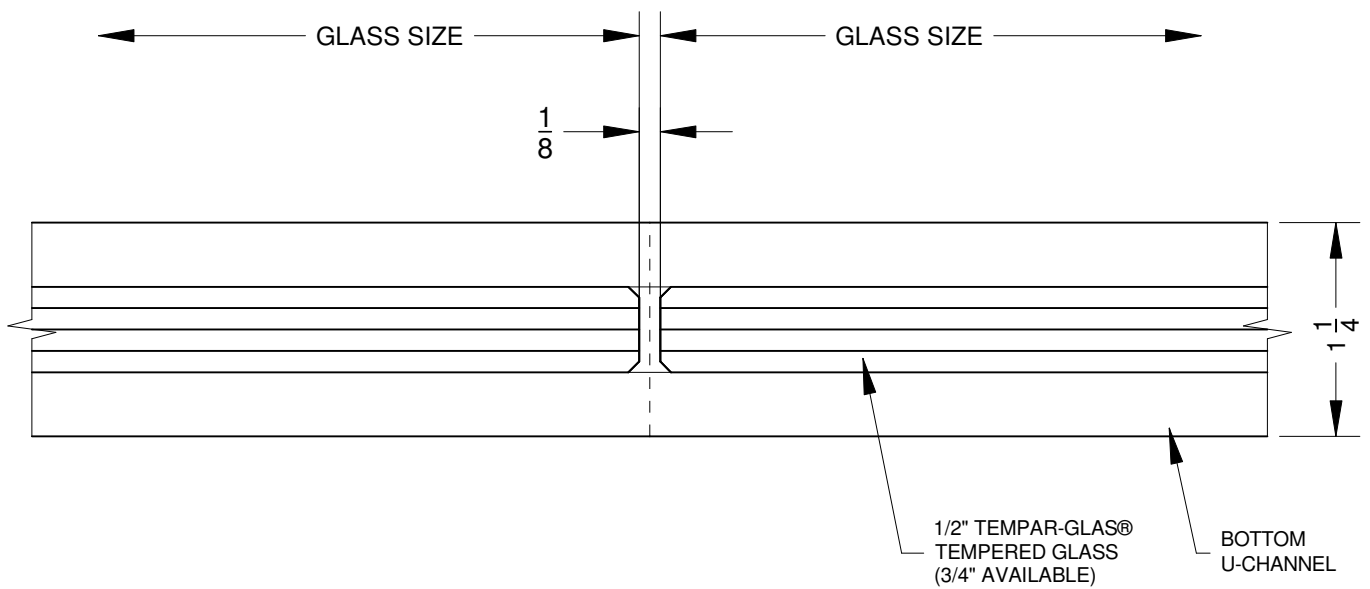
(B) - PLAN DETAIL AT MEETING SIDELIGHTS w/ U-CHANNEL
