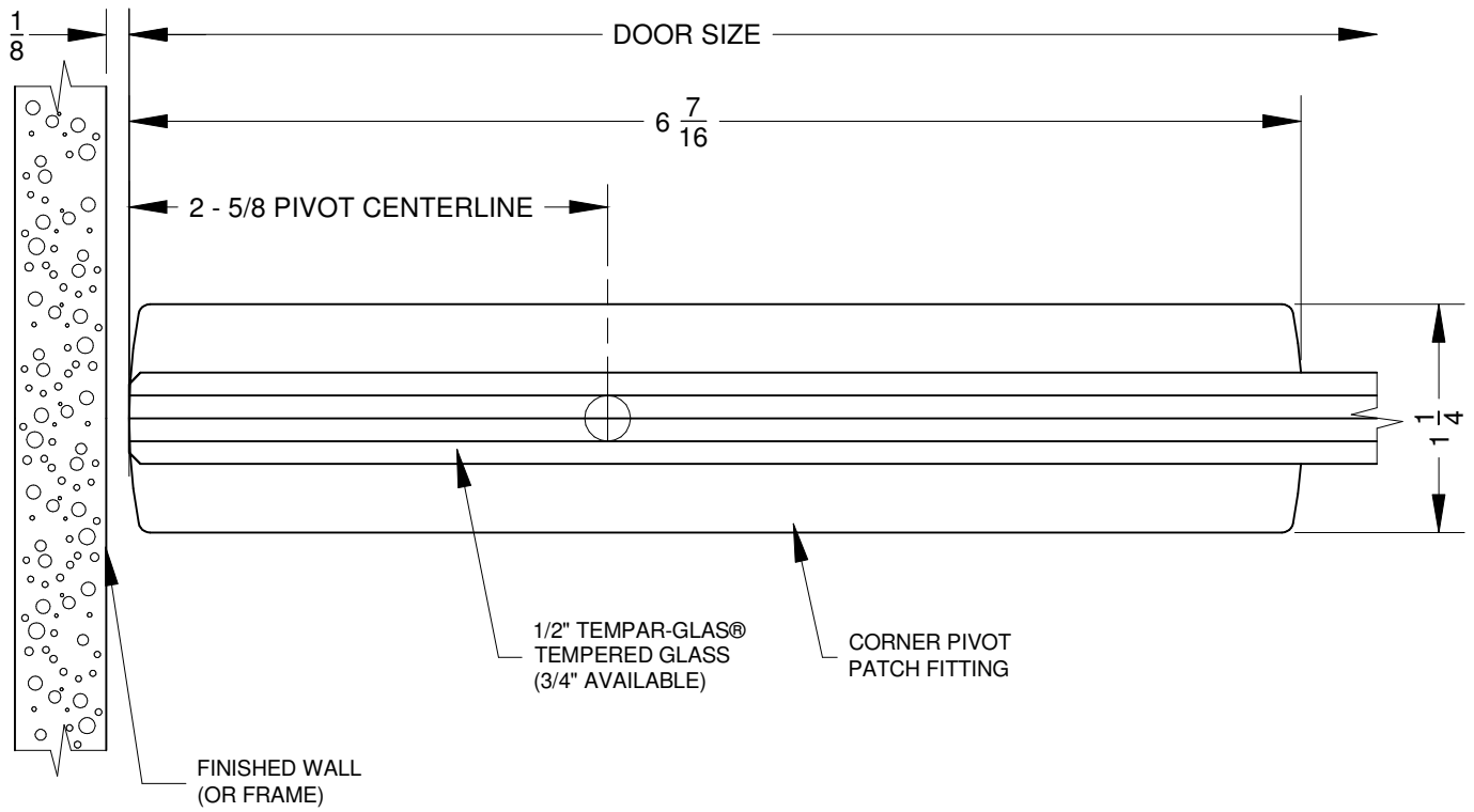
(A) - PLAN DETAIL AT WALL
