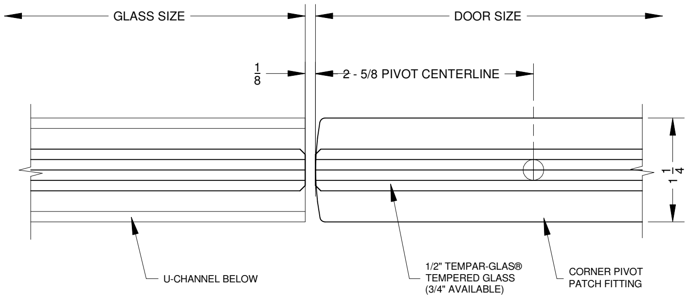
(B) - PLAN DETAIL AT SIDELIGHT
