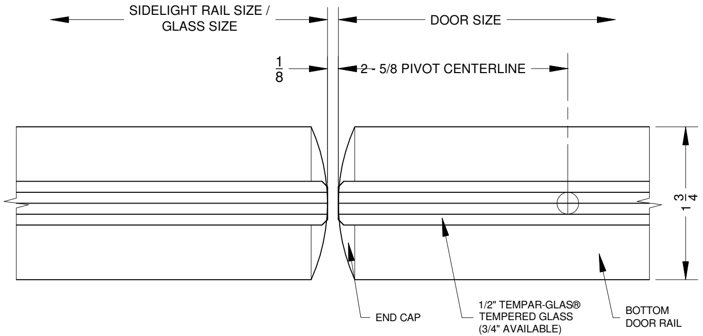
PLAN DETAIL AT SIDELIGHT
