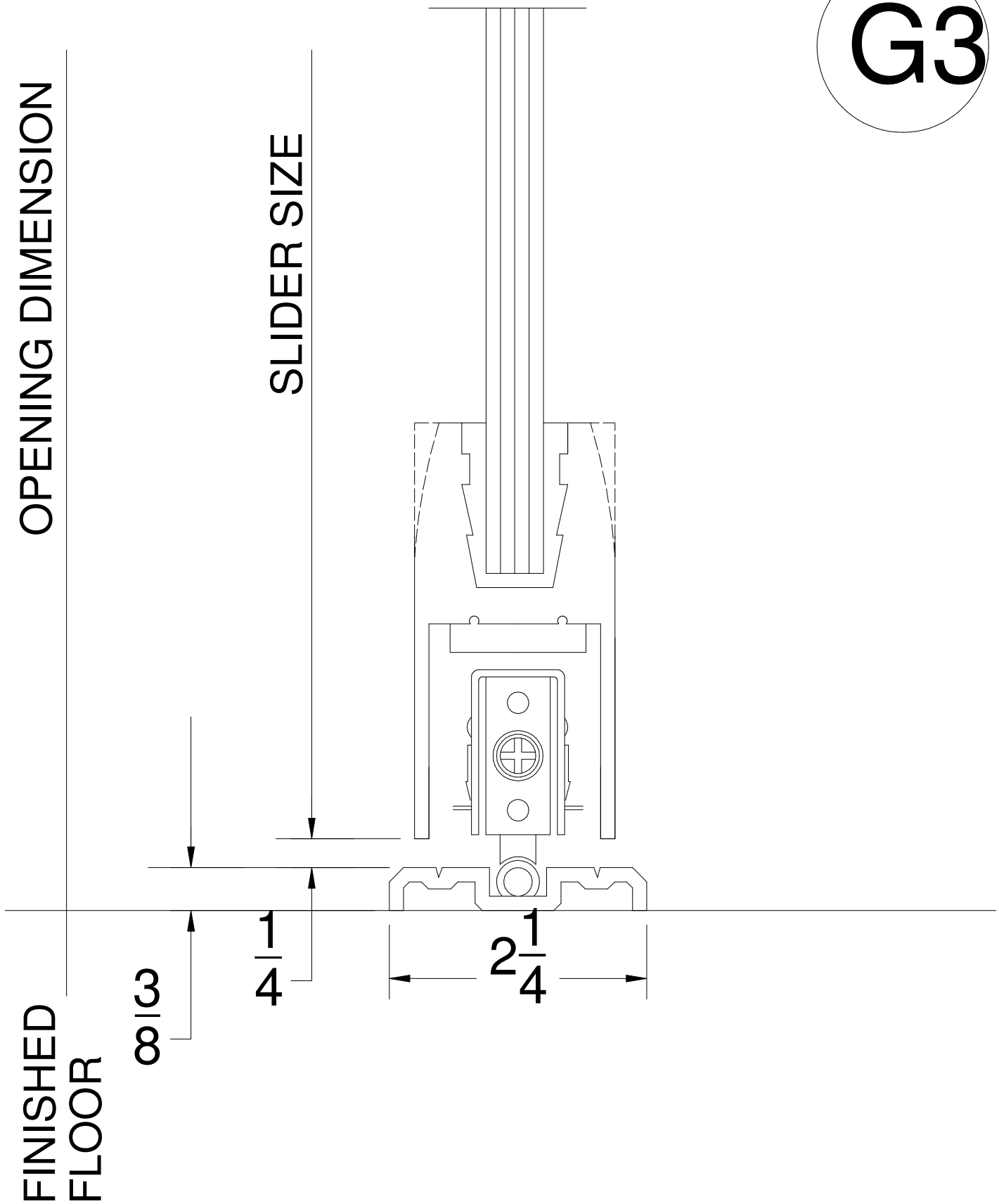
Sliding Panel Sill W/ Roller Track Mounted on Finished Floor
