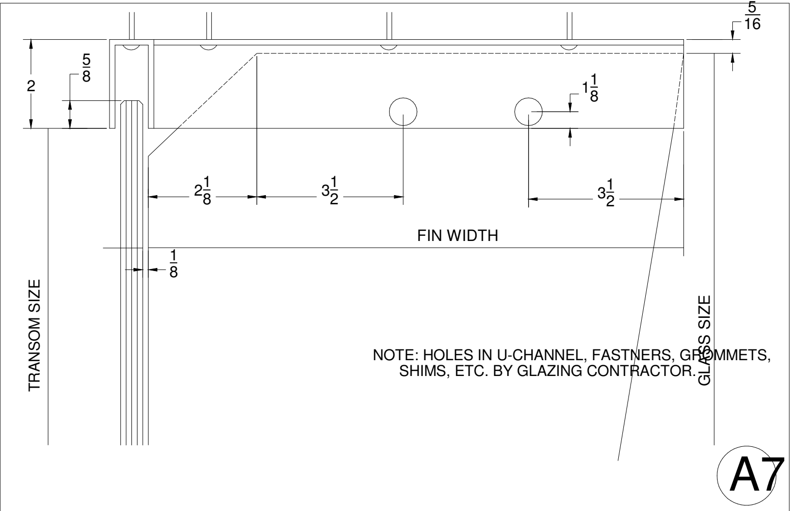
Section at Top of Fin (May be Surface Mounted or Recessed in Ceiling)
