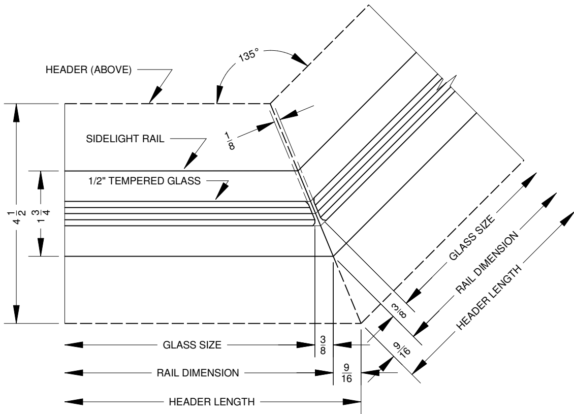
(A) - PLAN DETAIL w/ MITERED GLASS AND MITERED FRAME
