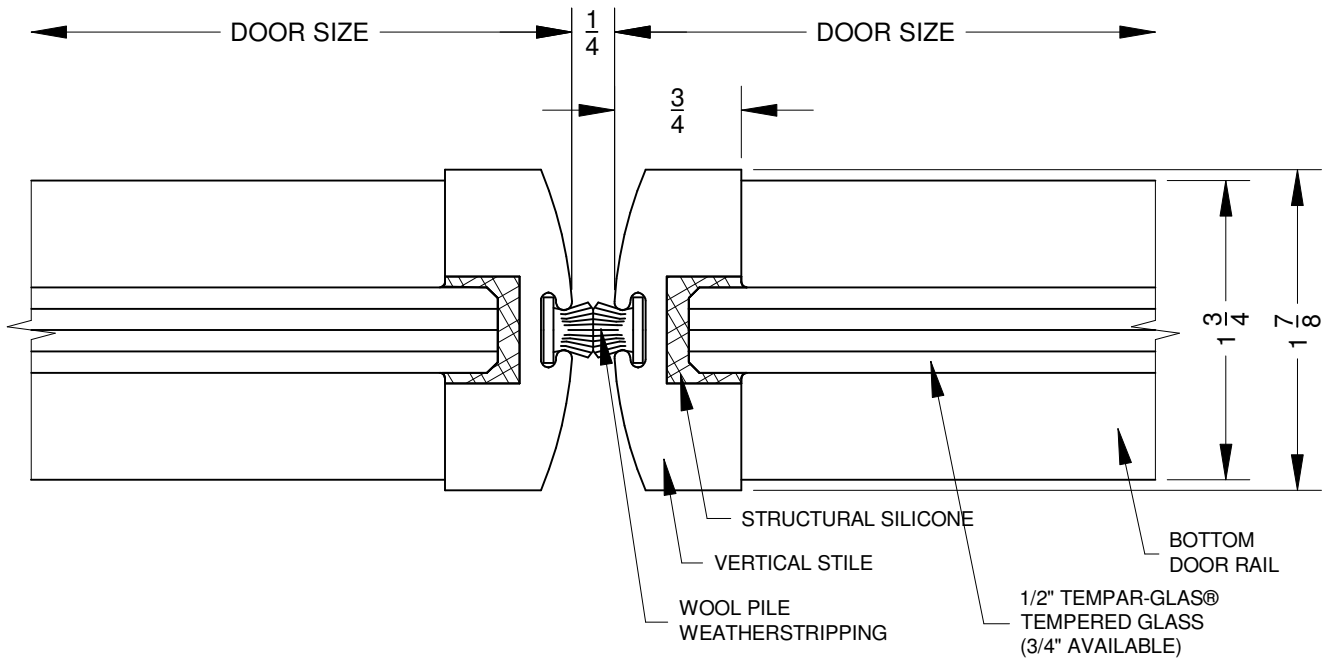
(B) - PLAN DETAIL AT MEETING STILES
