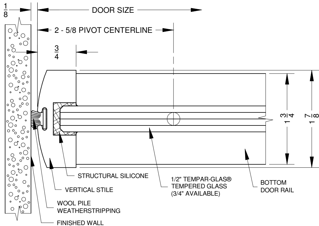
(A) - PLAN DETAIL AT WALL
